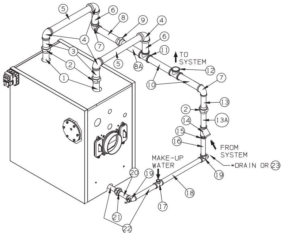
FIGURE 4: Dropped Header Gravity Return Diagram for FSZ160
