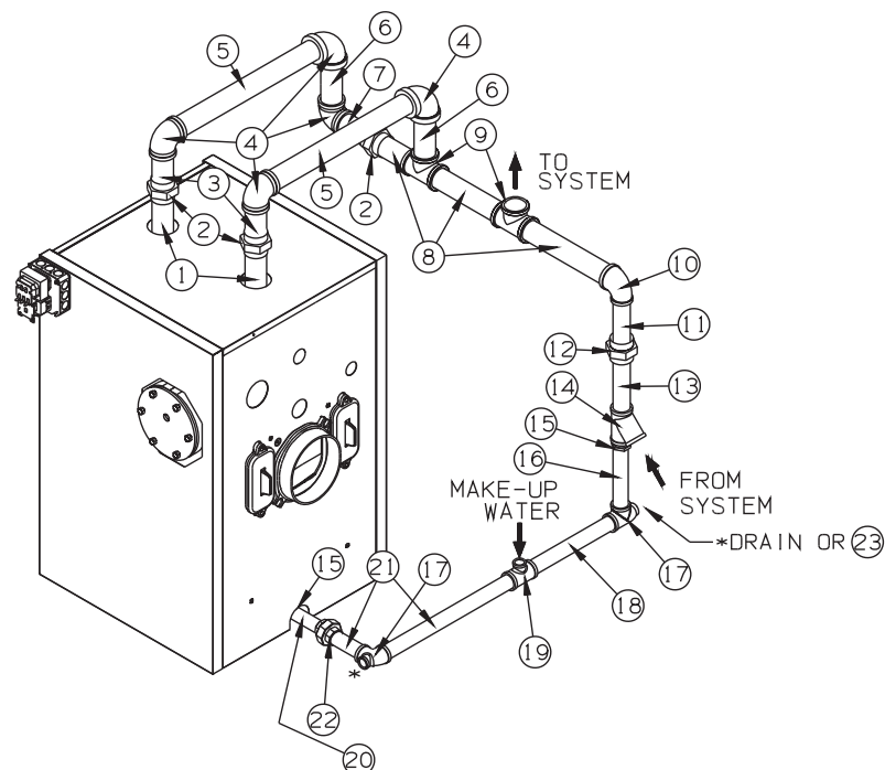
FIGURE 2: Dropped Header Gravity Return Diagram for FSZ080, FSZ100 and FSZ130
