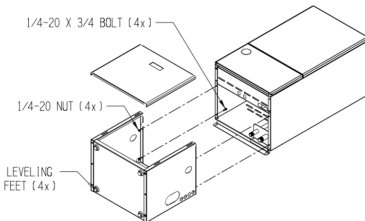
Figure 2: Assembling Pedestal to Boiler
