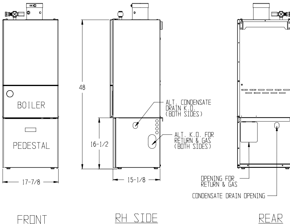
Figure 1: Basic Pedestal Configuration (Shown with Boiler Mounted)
